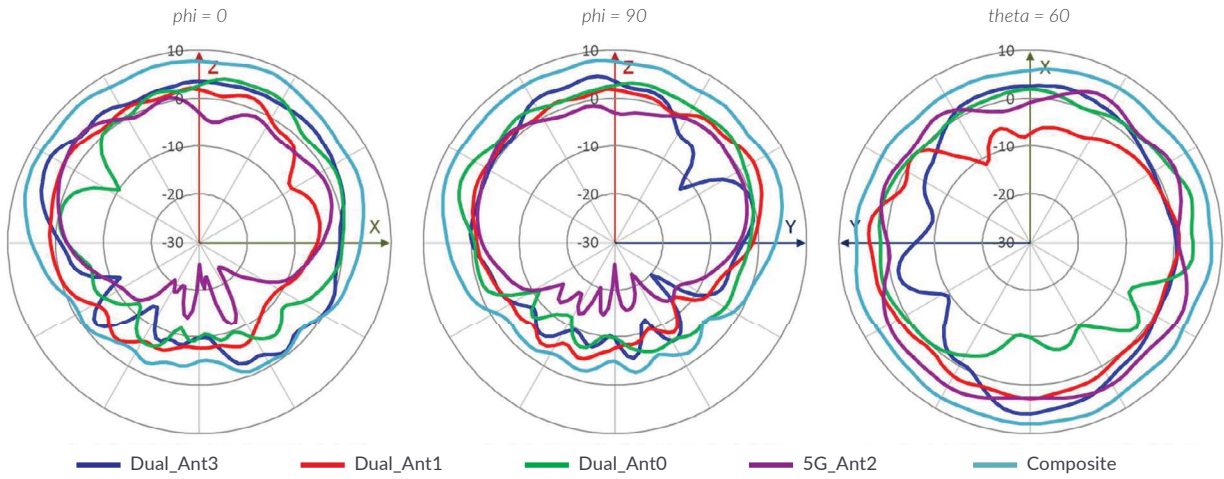
Wi-Fi @ 5150MHz (R0)
