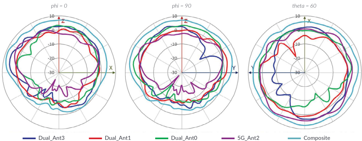
Wi-Fi @ 5850MHz (R0)
