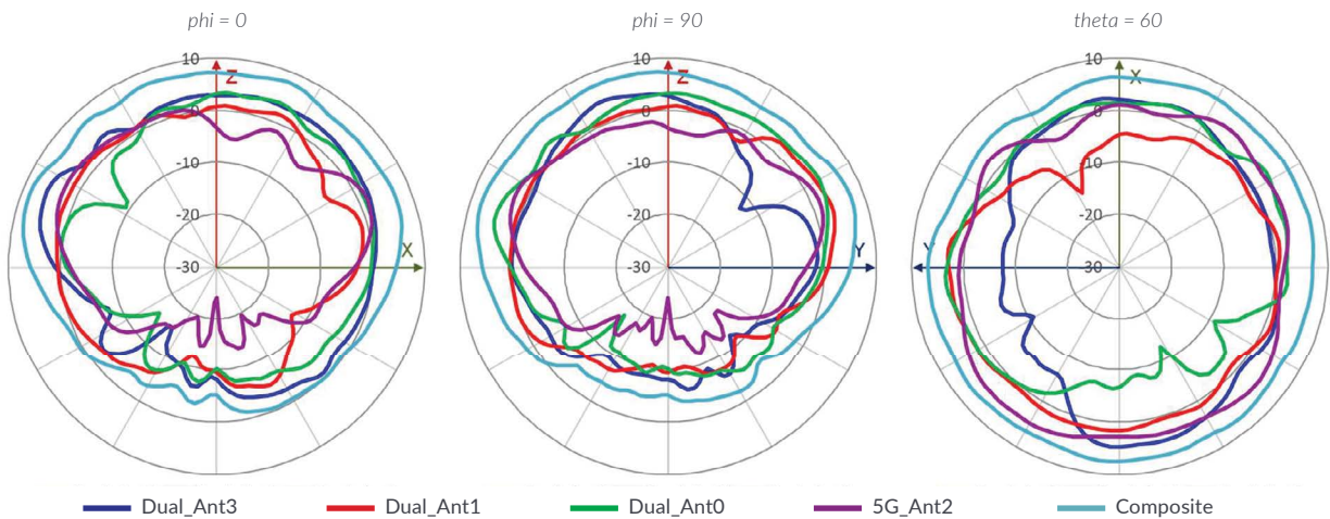
Wi-Fi @ 5550MHz (R0)
