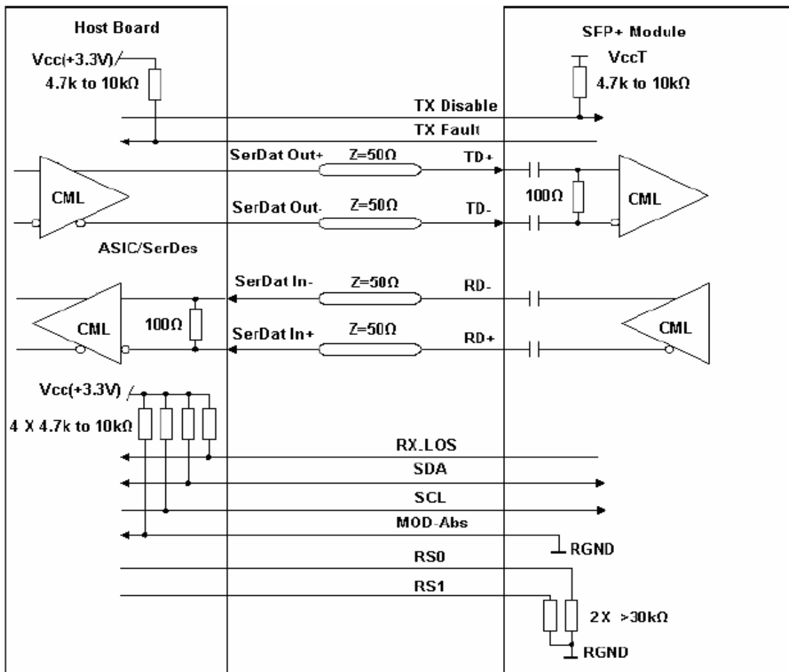
Recommended High-speed Interface Circuit
