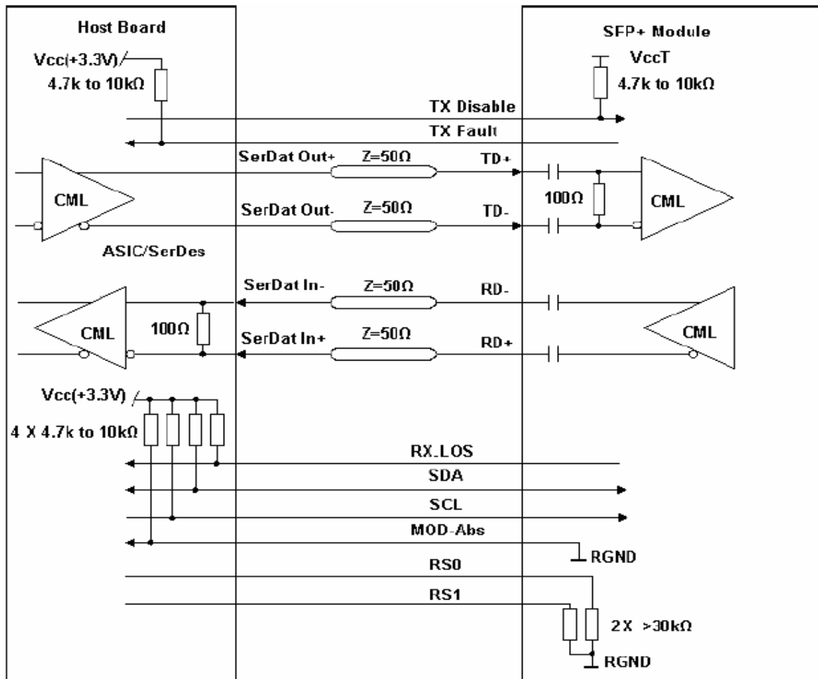
Recommended High-speed Interface Circuit
