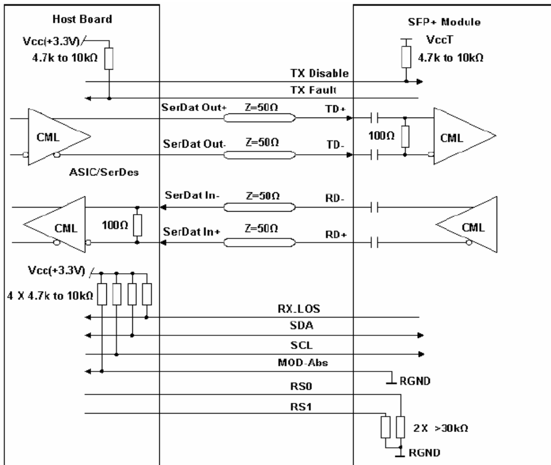
Recommended High-speed Interface Circuit
